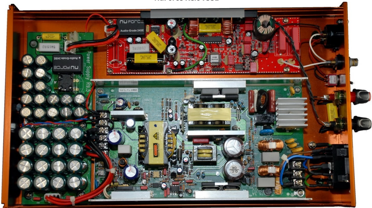
NuForce Ref9V3SE Innenleben
